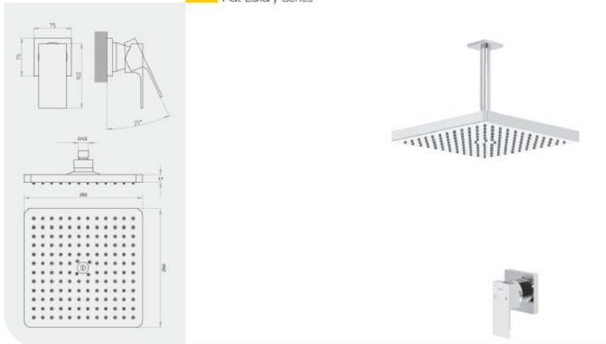
Shower Set, type 1 Flat Luxury Series
