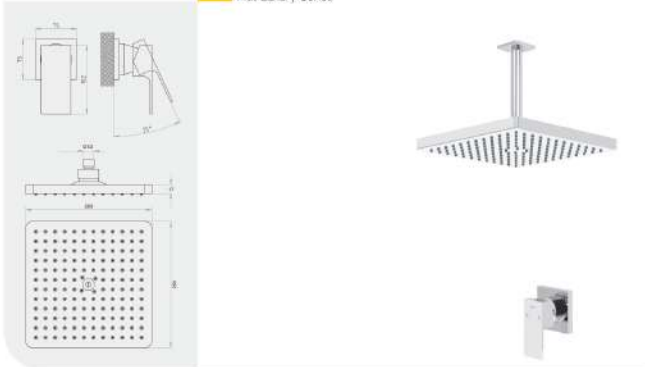
Shower Set, type 1 Flat Luxury Series
